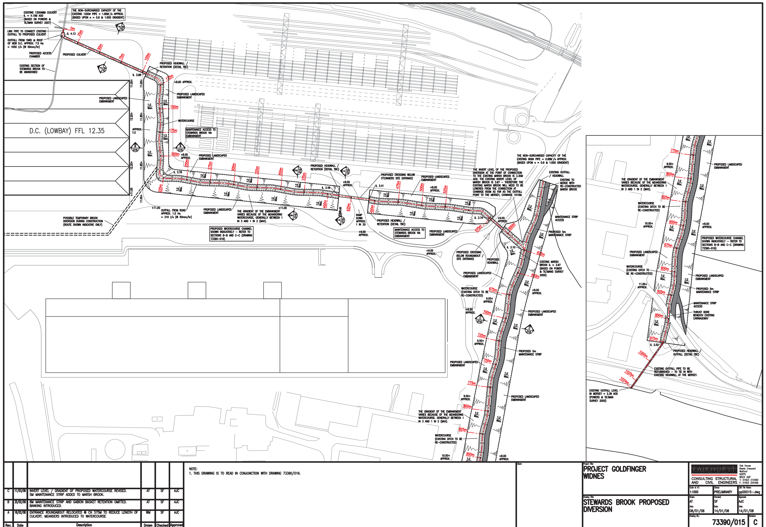
Title Figure 1.3: Proposed Steward's Brook Diversion
